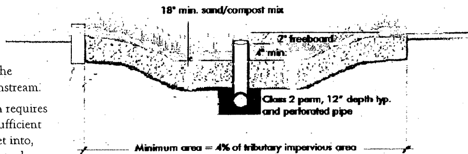
Drawing adapted from the Portland Stormwater Manual, 2002
